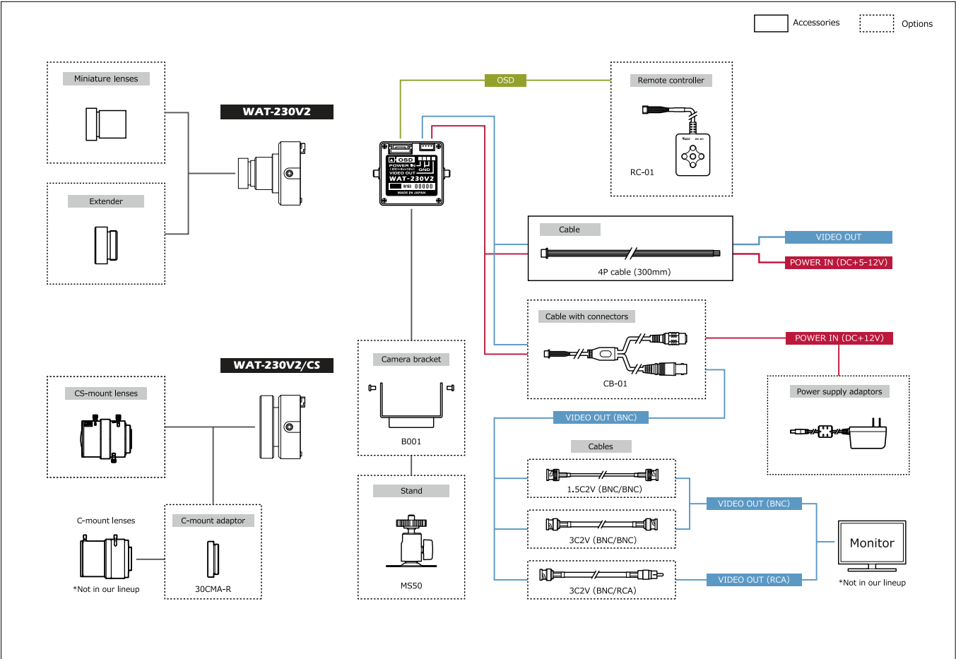
System diagram Representative connection example of the WAT-230V2 series
