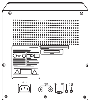
Rear Panel
