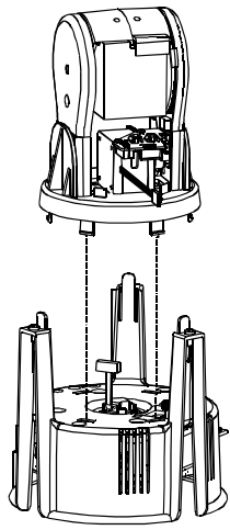
Base Assy. 0404-0008-01
