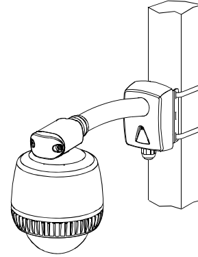
RHOWPA pole mount comes with the ROENDC end cap
