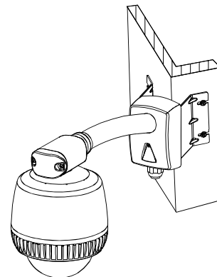
RHOWCA corner bracket only (shown with RHOLW mount)
